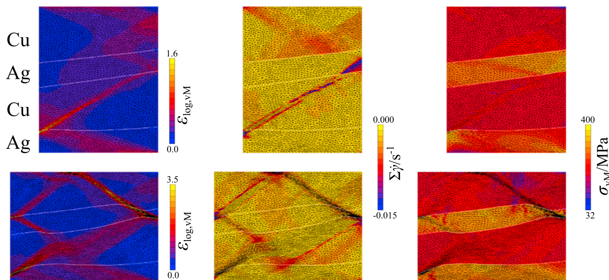
Fig. 27. Simulation results of equivalent logarithmic strain, sum of shear rates on the shear band systems and equivalent \text{CAUCHY} stress for the Copper-Silver bicrystal at 20% (top) and 40% (bottom) thickness reductions. Figure adopted from [241] with permission from Elsevier.
