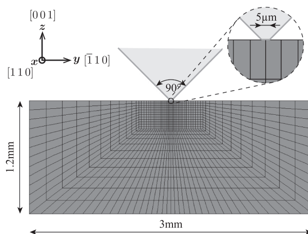
Fig. 16. Finite element mesh used for the simulation of wedge indentation. The indenter is modeled by two flat surfaces that have an inclination angle of 90° and a flat tip of 5 \mu\text{m} width. Figure adopted from [124,169] with permission from Elsevier.
